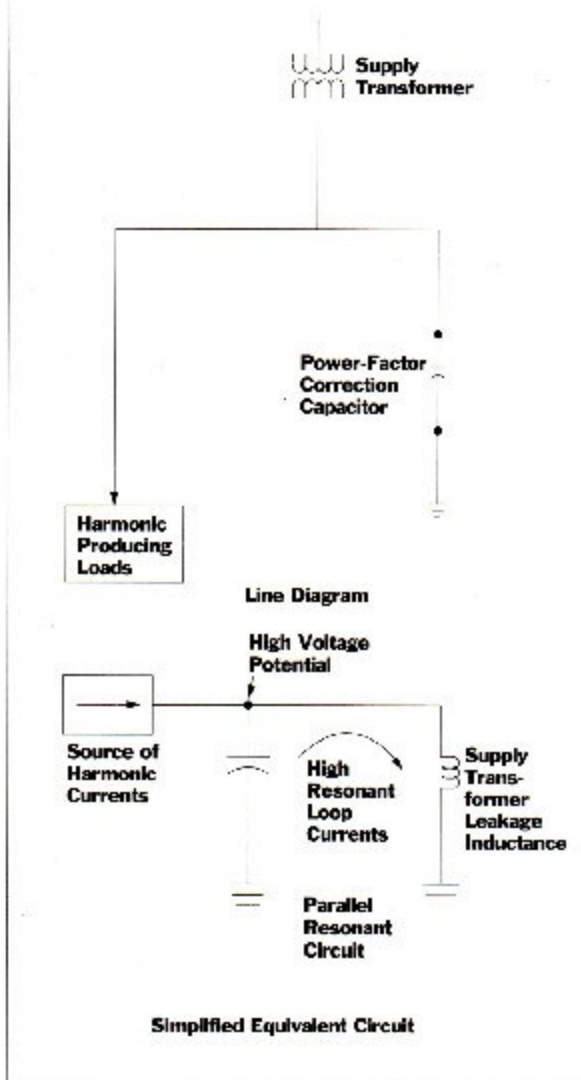
FIGURE 2 Harmonic Amplification Due to Resonance
