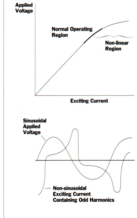
FIGURE 1 Transformer Excitation Curve and Waveforms in Non-linear Region
